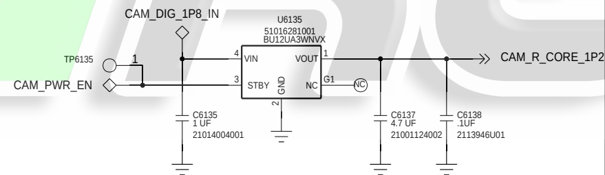
CAMERA CORE 1.2V
